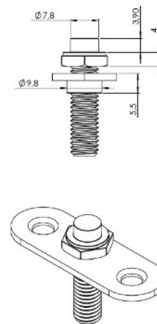
BOTTOM FITTING
